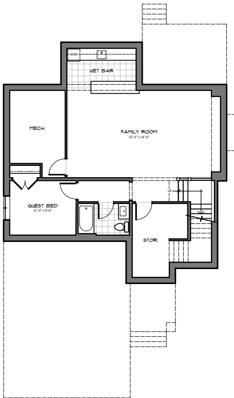
BASEMENT 750 FT 2
